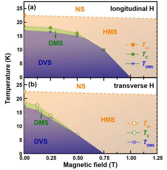
FIG. 4. Temperature-field phase diagrams for \text{EuFe}_2(\text{As}_{0.8}\text{P}_{0.2})_2 under an applied longitudinal (a) and transverse (b) magnetic field, respectively. T_{\text{C}} denotes the temperature below which the ferromagnetic correlations get established. T_{\text{sc}} denotes the superconducting transition temperature, which is supposed to be suppressed very slowly under 2 T for \text{EuFe}_2(\text{As}_{1-x}\text{P}_x)_2 [15]. NS, HMS, DMS, and DVS denote the normal state above T_{\text{sc}} , the homogeneous Meissner state in between T_{\text{sc}} and T_{\text{C}} , the domain Meissner state in between T_{\text{C}} and T_{\text{DMS}} , and the domain vortex-antivortex state below T_{\text{DMS}} , respectively. T_{\text{DMS}} is determined according to the temperature at which the magnetic SANS intensity in Figs. 2(c) and 2(d) displays an additional feature and the I(q) profiles show a clearly identified double-bump structure.
