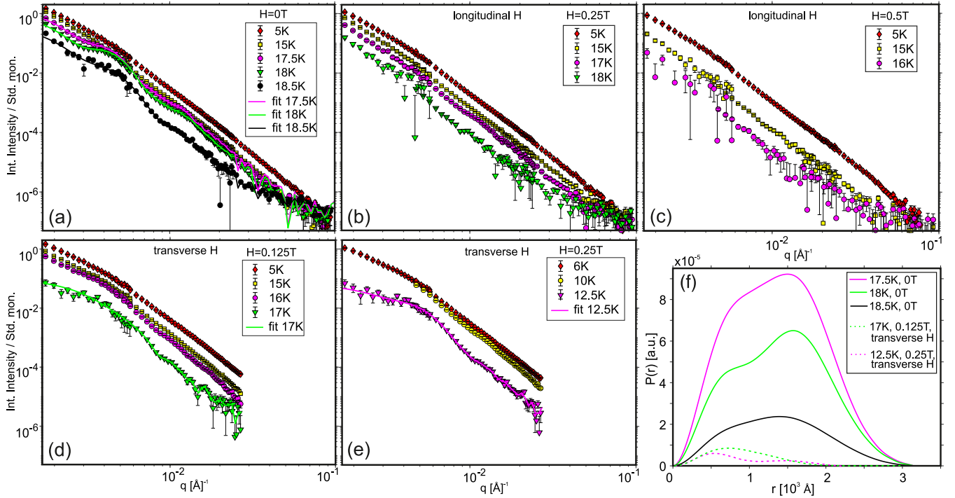
FIG. 3. The q dependencies of the radially integrated magnetic SANS intensity at different temperatures in zero magnetic field (a), a longitudinal field of H_l = 0.25\text{ T} (b) and H_l = 0.5\text{ T} (c), and a transverse field of H_t = 0.125\text{ T} (d) and H_t = 0.25\text{ T} (e). The I(q) curves with a double-hump feature collected at the intermediate temperatures just below T_C , for the zero-field and transverse-field case, were fitted using the IFF method, as the solid lines in (a), (d), and (e) represent. (f) shows the extracted real-space pair distance distribution function P(r) , revealing the existence of the DMS at intermediate temperatures closely below T_C .
